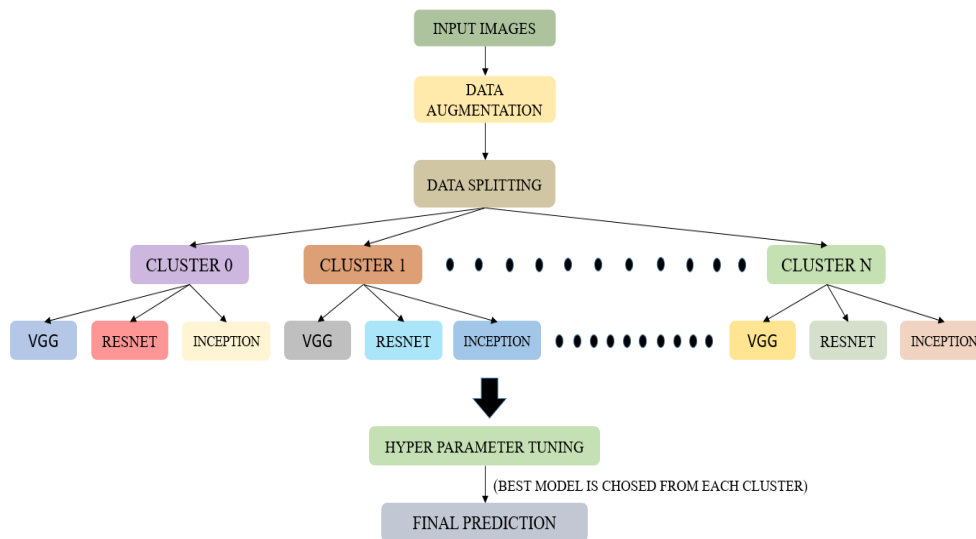
Fig.1. Proposed Framework.
