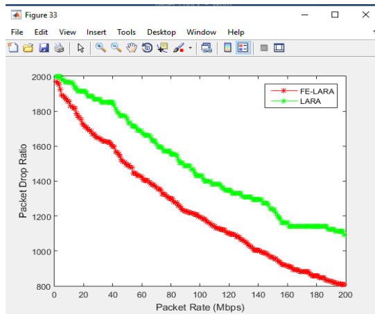
Fig. 12. Analysis Graph for packet drop ratio of LARA and FE- LARA
