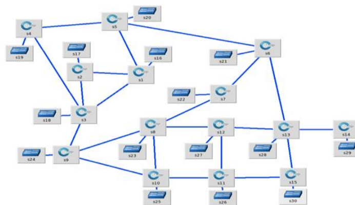
Fig.2. Hybrid SDN Network with 15 Open Flow Switches.
