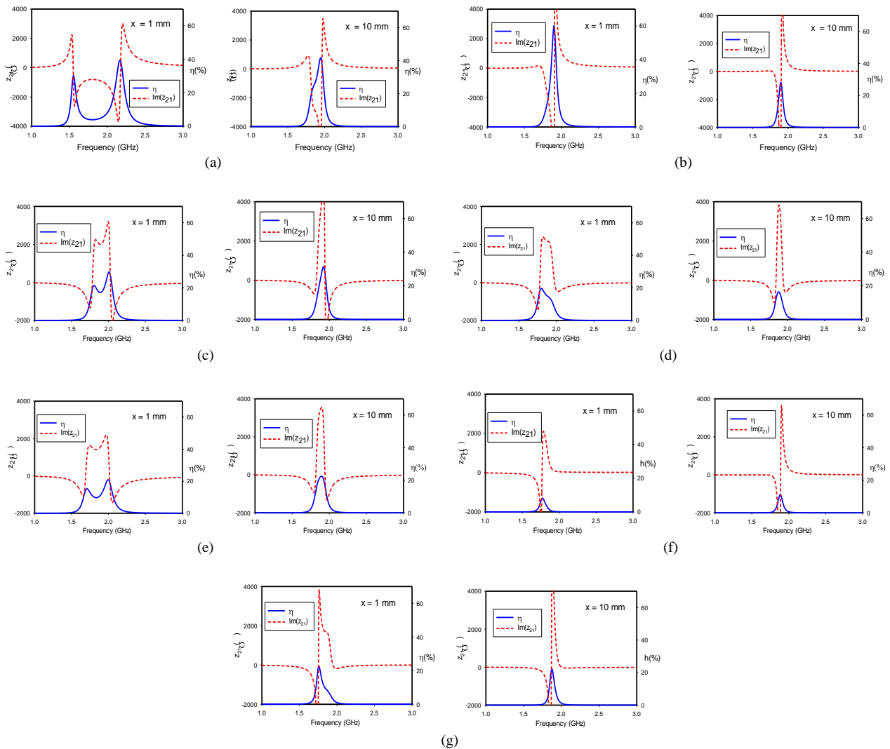
Fig. 4. Transfer efficiencies and through impedance of edge-coupled dimer for various rotational orientations: (a) ‘AC’, (b) ‘DD’, (c) ‘CA’, (d) ‘CD’, (e) ‘BD’, (f) ‘BC’, (g) ‘CC’
