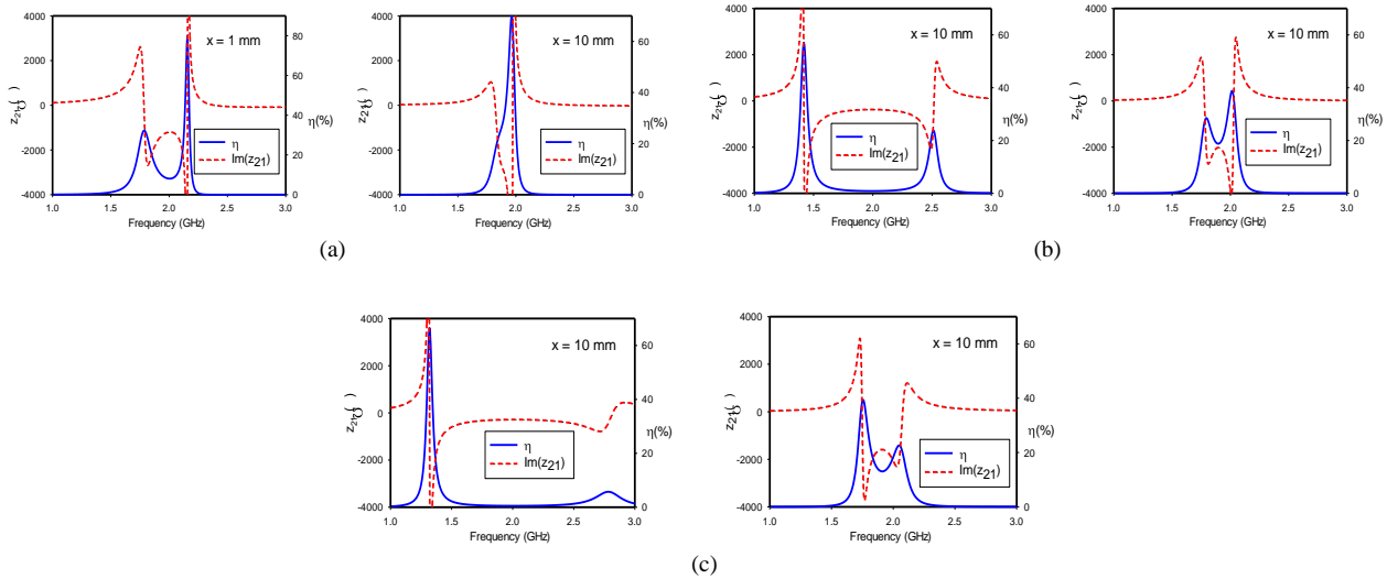
Fig. 5. Transfer efficiencies and through impedance of broadside-coupled dimer for various rotational orientations: (A) ‘AA’, (b) ‘BA’, (c) ‘CA’
